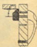
Catch Applied to Flush or Overlapping Door Using "F" Strike Applied to Under Side of Shelf. Suggested for Double Door Installation.
