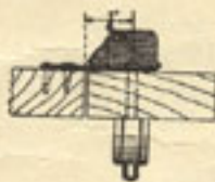
Catch Applied to Flush Door Using "F" Strike with Formed End broken Off
