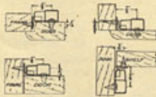
No. E9708 Cabinet Maker Pack
