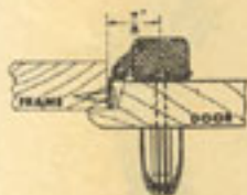
Catch Applied to Overlapping Doors Using "D" Strike
