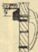
Catch Applied to Flush or Overlapping Door Using "F" Strike Applied to Under Side of Shelf. Suggested for Double Door Installation.
