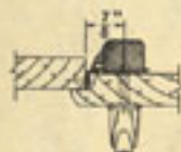
Catch Applied to Overlapping Doors Using "D" Strike
