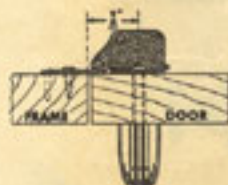
Catch Applied to Flush Door Using "F" Strike with Formed End broken Off
