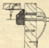
Catch Applied to Flush or Overlapping Door Using "F" Strike Applied to Under Side of Shelf. Suggested for Double Door Installation.
