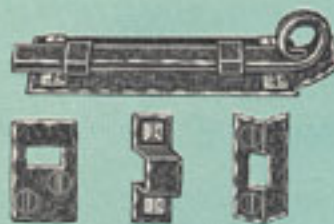
No. W1190 BOLT Three sizes: 3", 4", and 6" Furnished with universal, angle and surface strikes. One in envelope with pyramid screws All sizes packed 1 dozen, weight 3": 3 lbs., 4": 4 lbs., 6": 5 lbs.
